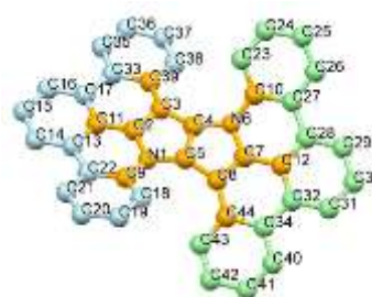
Figure 4. Geometry of 1 in the relaxed S_1 state (H atoms omitted) with the atom numbering used in the definition of geometrical parameters in Table 2 and the colour code for the definition of the regions in Table 3: left (light blue), centre (orange), right (green).
