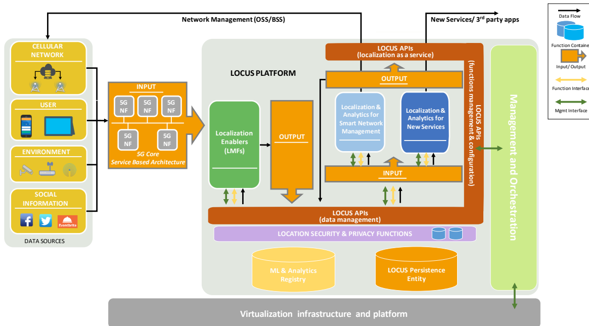
Fig. 2. LOCUS Architecture
