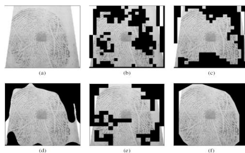
Figure 3. Segmentation results using different methods in DB2: (a) Original image, (b) SVM [11], (c) K-means [13], (d) MP [17], (e) ATC [19], (f) Proposed method
