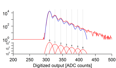
Figure 3: MPPC finger plot. Peaks represent 1, 2, 3, ... photo electrons respectively.
