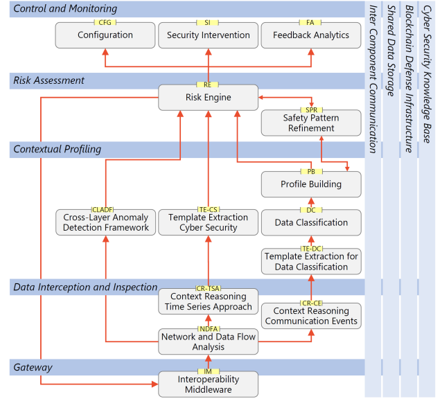
Fig. 1. GHOST system architecture
