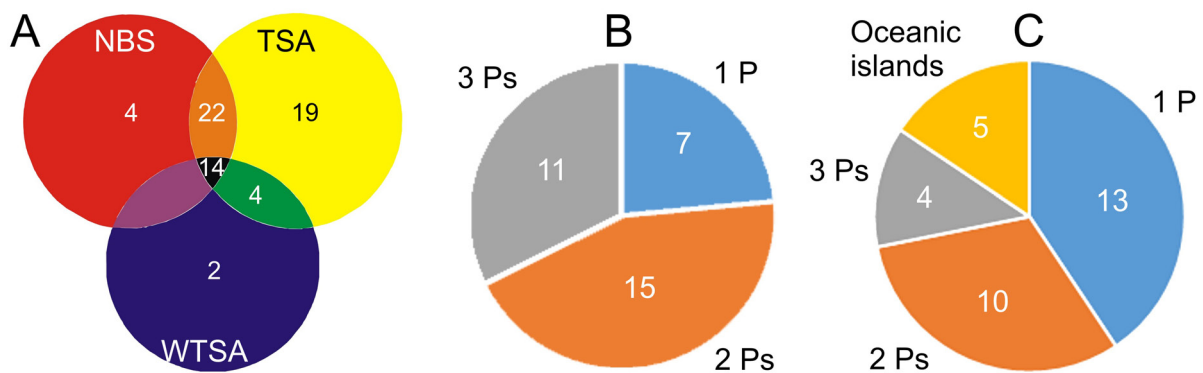
Fig. 82. Distribution of triphorids in Brazil according to the marine provinces of Spalding et al. (2007). A. Number of species in each province: NBS = North Brazil Shelf; TSA = Tropical Southwestern Atlantic; WTSA = Warm Temperate Southwestern Atlantic. B. Range of planctotrophic species in Brazil; ‘ n ’ Ps refer to species present in n provinces. C. Range of lecithotrophic species in Brazil (those exclusively living near oceanic islands were set apart).
