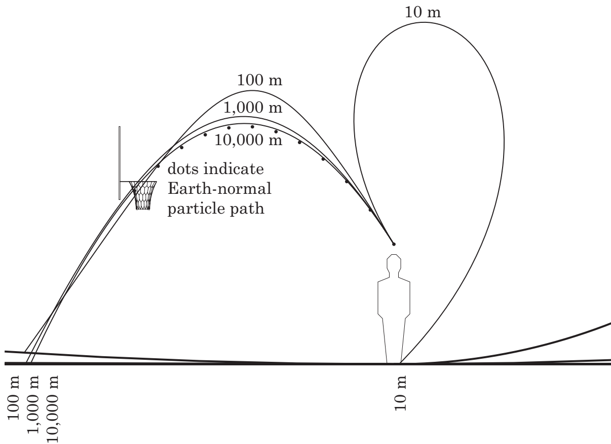
FIGURE 1. Basketball in 1-g centripetal acceleration, shooting from 2 m above the free-throw line; from Hall [48]. The curves indicate particle paths in rotating habitats with floor radii of 10 m, 100 m, 1,000 m, and 10,000 m. (Closer under the net with a more “vertical” shot, the path is apt to curve backward even in a 100-m radius habitat. See Hall [48].)
