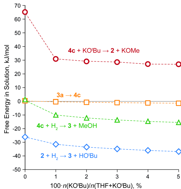
Figure 6. Concentration-dependent free energy changes for the key elementary steps at the reaction conditions (373K, 50 bar \text{H}_2 ) computed using a realistic COSMO-RS solvent model.
