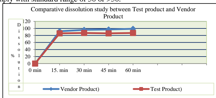
Fig. 8: Graphical presentation of comparative dissolution study between test product and vendor product.
