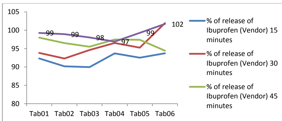
Fig. 10: Graphical presentation of % release profile of Ibuprofen (vendor).
