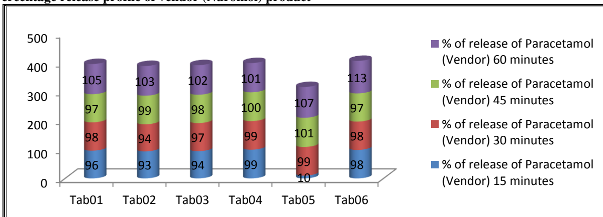
Fig. 9: Graphical presentation of percentage release profile of Paracetamol (vendor).
