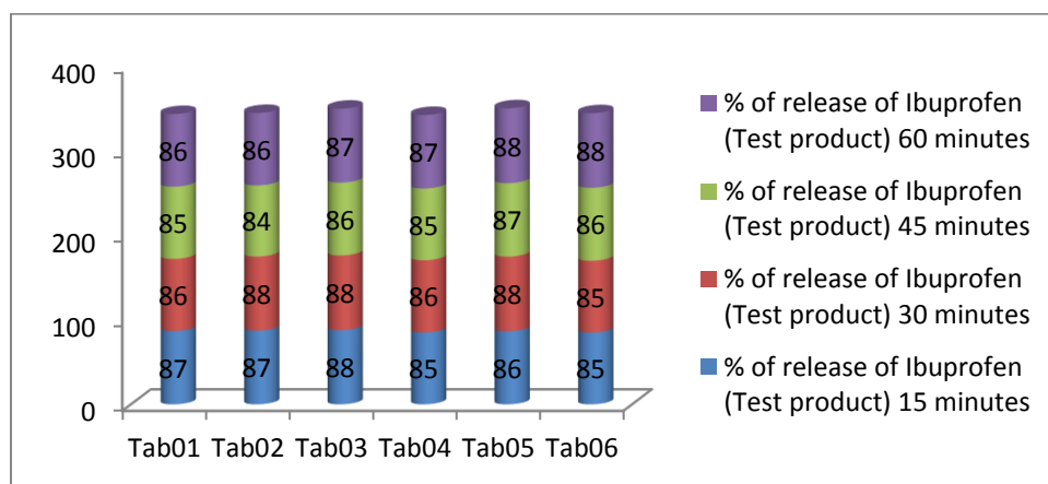
Fig. 12: Graphical presentation of percentage release profile of Ibuprofen (test product).
