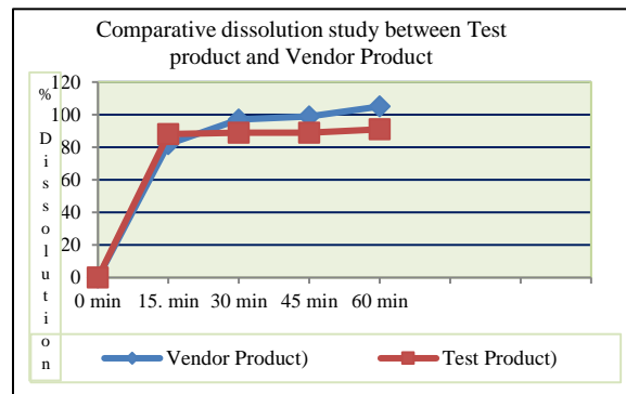
Fig. 7: Graphical presentation of comparative dissolution study between test product and vendor product.
