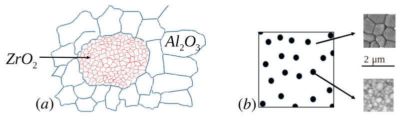
Figure 3: a) Sketch of Alumina-Zirconia Ceramic Matrix Composite. b) Meso and Micro scales of Al_2O_3 - ZrO_2 CMC composite.
