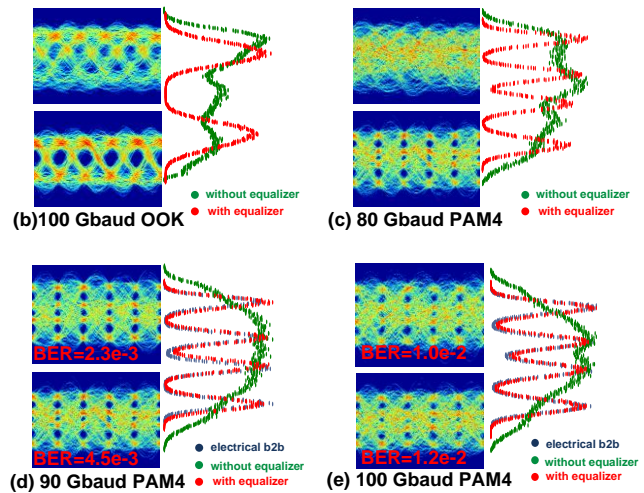
Fig. 4. (a) BER curves for the OOK and PAM-4 signals for b2b and 400 meters, (b)-(c) eye diagram and histograms at optical b2b without and with DFE at 8 dBm, and (d)-(e) eye diagrams and histograms with DFE for electrical b2b (top) and optical b2b (bottom) at 8 dBm.
