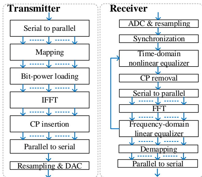
Fig. 5. A typical DSP routine of the DMT transmitter and receiver. FFT / IFFT: fast Fourier transform / inverse FFT; CP: cyclic prefix.
