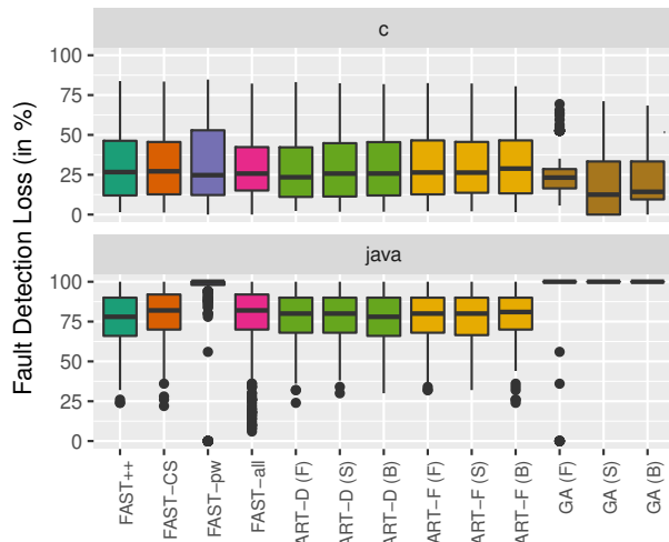
Fig. 2: FDL for the test suite reduction approaches (in %).
