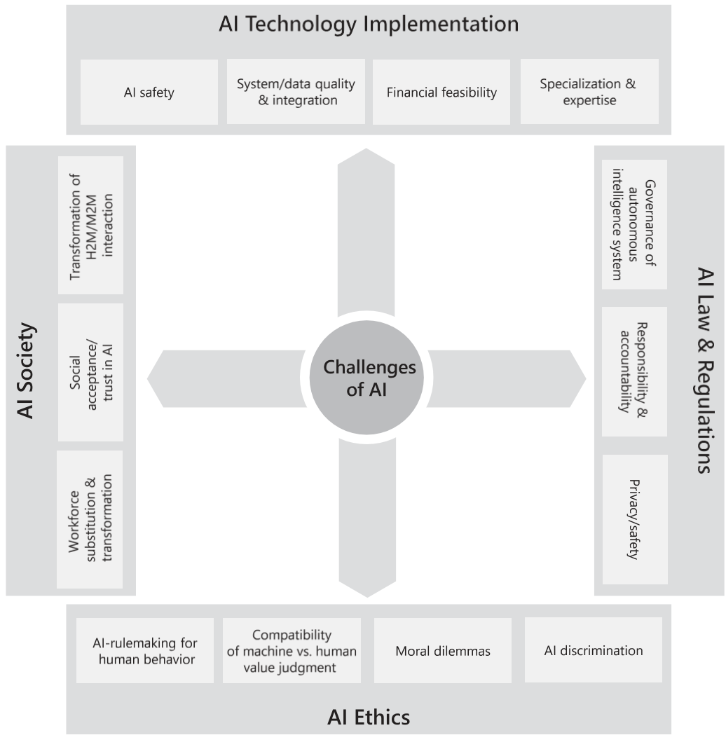
Figure 1. Four-AI-challenges model.
