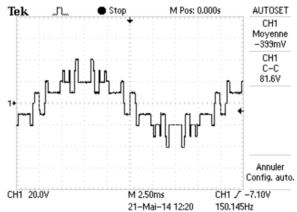
Fig. 11 Phase voltage (Va) of the used inverter
