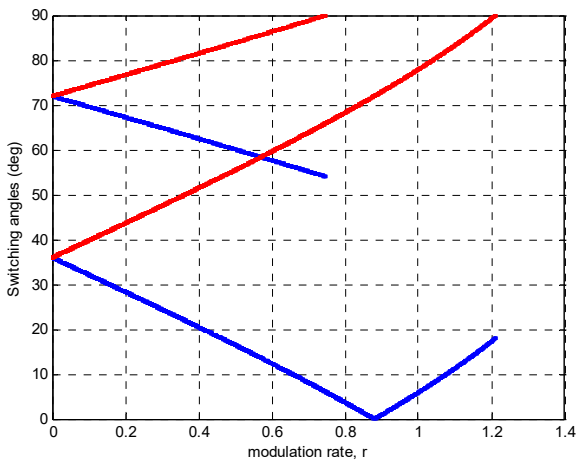
(a) Two switching angles to eliminate h_5 for three level inverter S_i = [1, -1]
