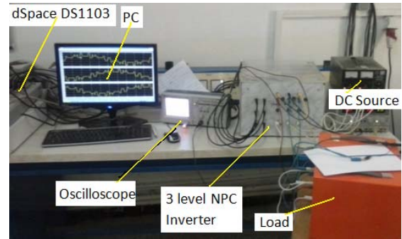
Fig. 9 Test work-bench
