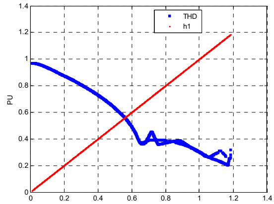
(a) Voltage THD and h_1
