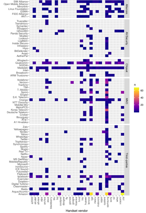
Figure 2: Permissions defined by AV firms, MNOs, chipset vendors and third parties, requested by pre-installed apps.
