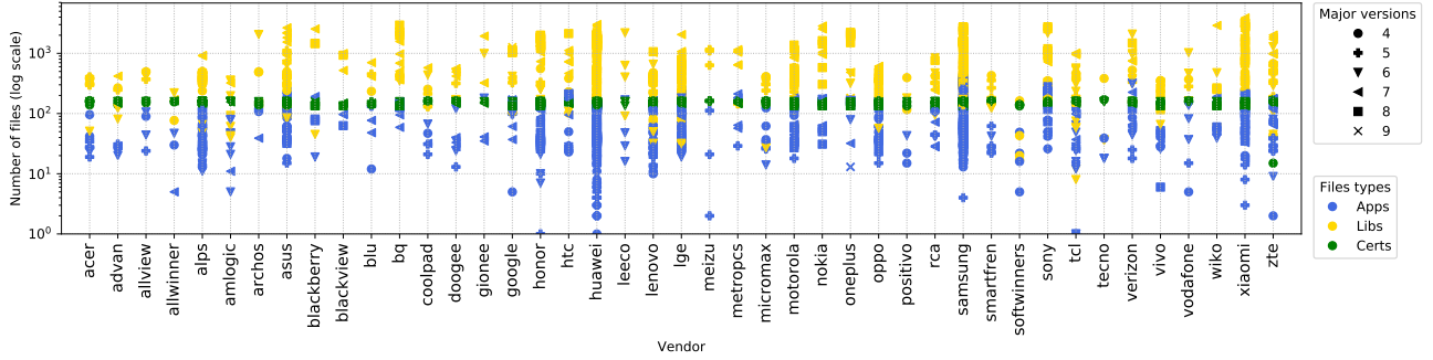
Figure 1: Number of files per vendor. We do not display the vendors for which we have less than 3 devices.
