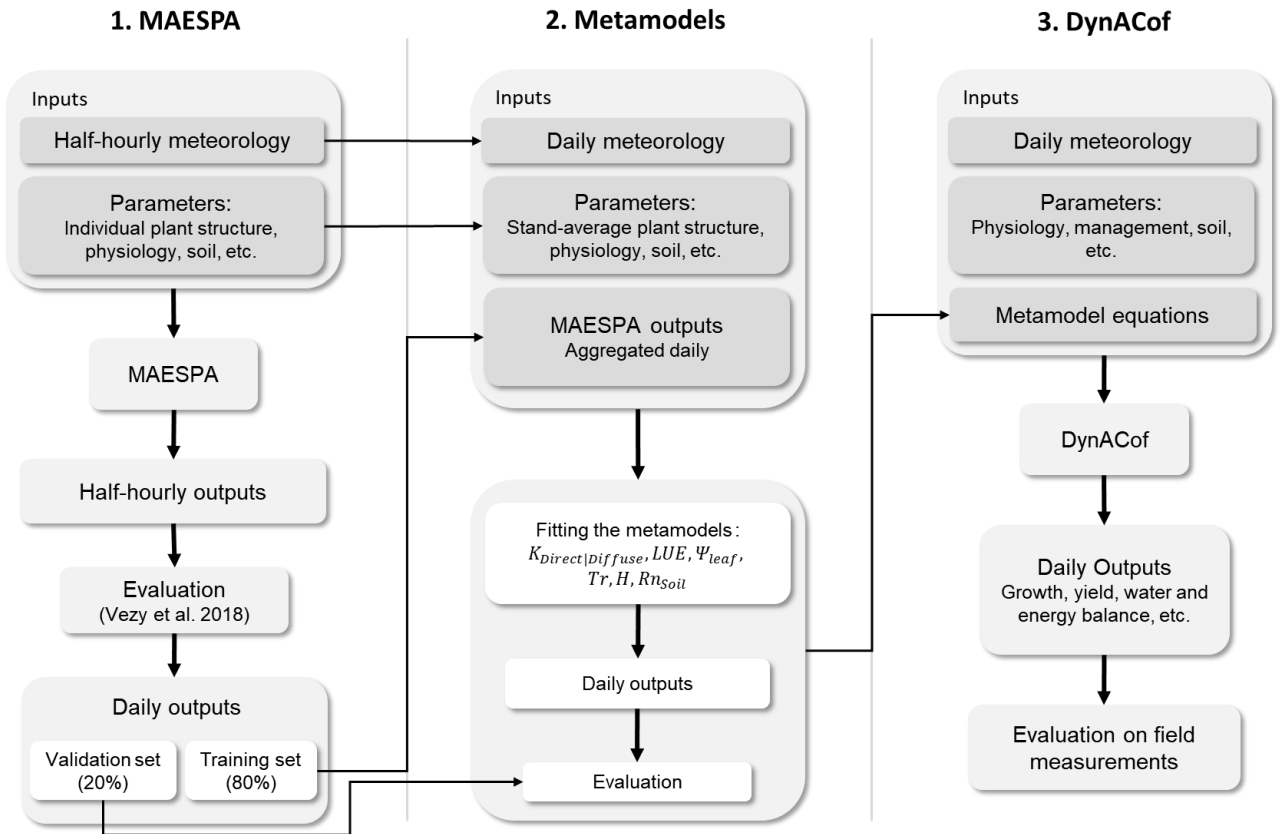
Figure 1. Flowchart of the three-step metamodeling approach. 1/ The resolution for stand simulations in MAESPA was the individual tree and the half-hourly time step. 2/ The metamodels were fitted using inputs (meteorology and parameters) at daily and stand scale used as predictors to model the MAESPA outputs integrated at daily and stand-scale (training set, 80% of the data). The metamodels were evaluated on the validation set (20% of the data). 3/ The metamodel equations were injected into DynACof.
