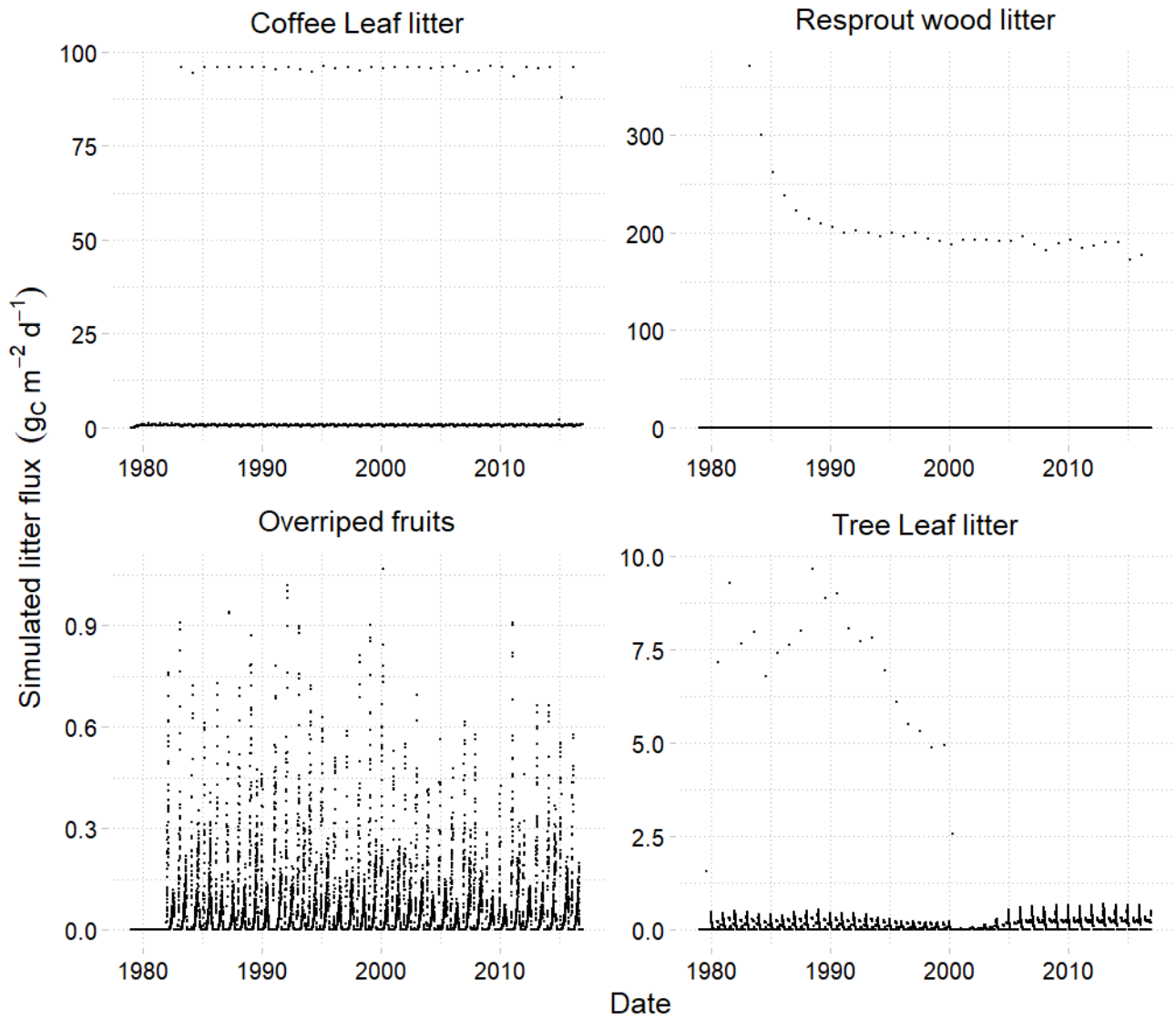
132 133 Figure D.4. Simulated litter fluxes for the compartments with the highest contribution for the coffee (leaf, resprout wood, fruits) 134 and the shade tree (leaf).
