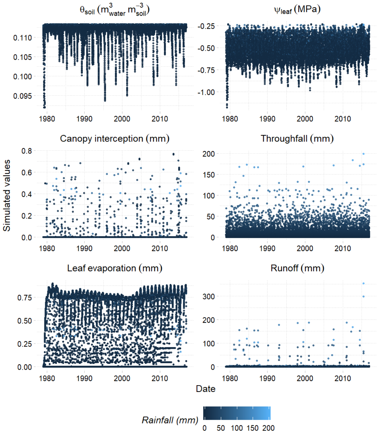
108 109 Figure D.2. DynACof outputs related to the water balance at daily time-scale and plot scale for the period starting from 1979- 110 01-01 until 2016-12-31. \theta is the volumetric water content for the full soil profile, and .
