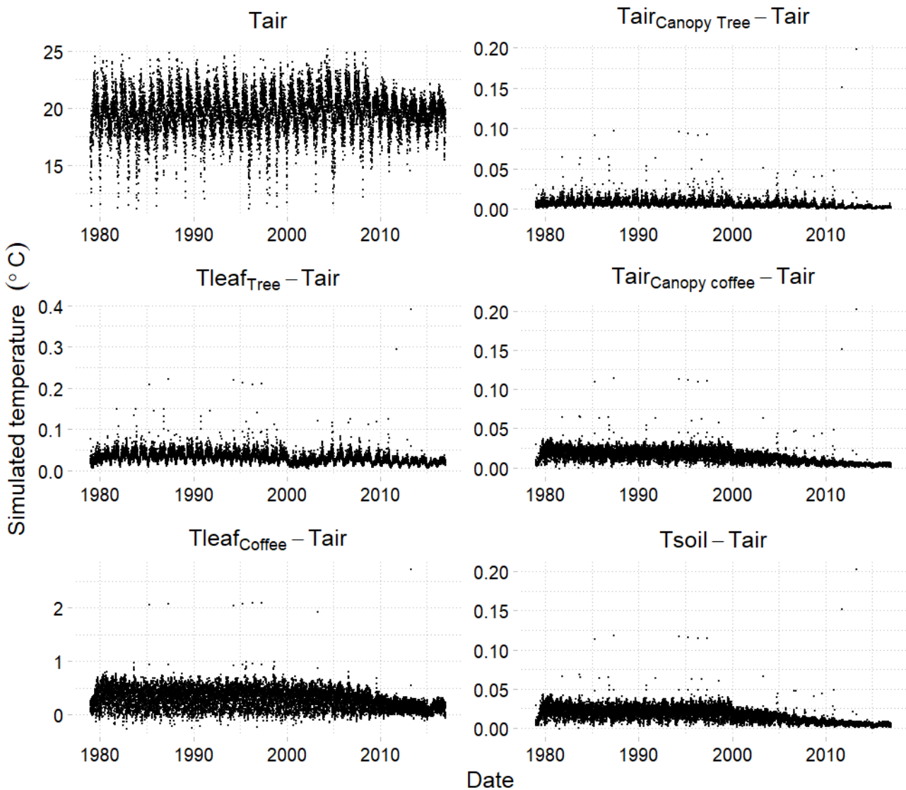
119 120 Figure D.3. Input ( T_{air} ) and simulated temperatures. The simulated temperatures are presented as the difference between the 121 simulated temperature and the input T_{air} for easier assessment.
