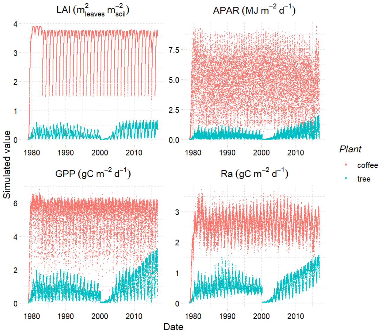
102 Figure D.1. Comparison of dynamic outputs from DynACof between shade tree and coffee for leaf area index (LAI), absorbed 103 photosynthetically active radiation (APAR), gross primary productivity (GPP) and autotrophic respiration (Ra) starting from 104 1979-01-01 until 2016-12-31. 105
