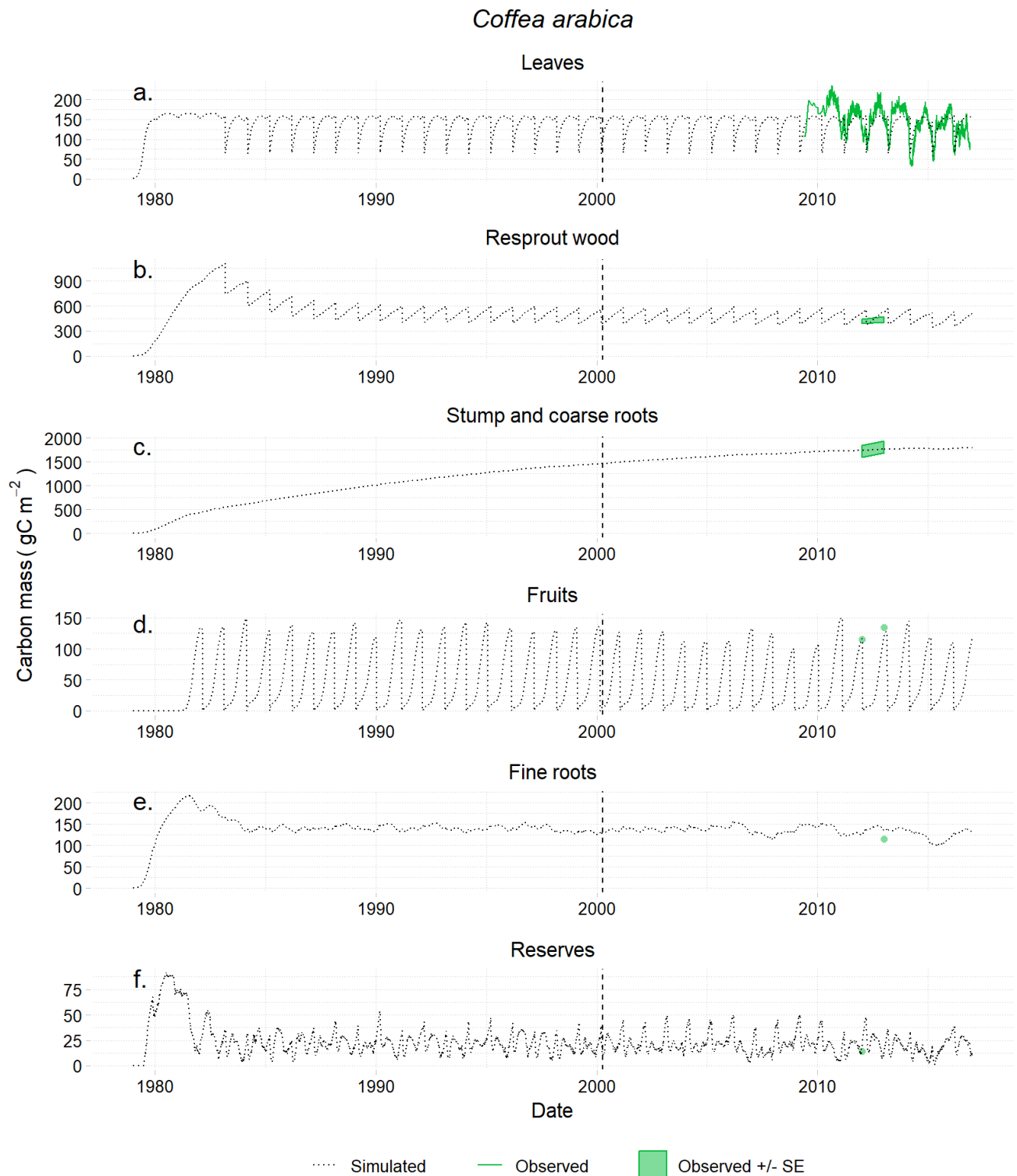
Figure 5. Simulated coffee plant carbon biomass per organ (dotted lines) over a full plantation cycle (1979-2016), compared to measured biomass (green dots: one observation, green lines: continuous measurement and polygon: mean observation +/- SE). a/ Simulated leaf C mass compared to measured NDVI calibrated using LAI2000, and converted into dry mass using leaf SLA and dry mass to carbon mass ratio (Taugourdeau et al., 2014), see Table 1; b/ Simulated wood C mass from branches compared to average +/-SE measured by Charbonnier et al. (2017); c/ Simulated C mass in stump and coarse roots compared to measured stump C mass +/- SE in Charbonnier et al. (2017) + measured perennial root C mass from Defrenet et al. (2016); d/ Simulated fruit dry mass compared to values measured by Charbonnier et al. (2017) for 2011 and 2012 at harvest; e/ Simulated fine roots C mass compared to a 2011 measurement by Defrenet et al. (2016); and f/ Simulated reserves compared to reserves measured by Cambou (2012), assumed to represent the minimum value of the year.
