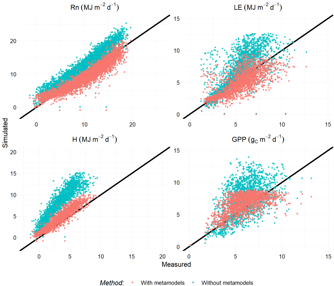
86 87 Figure C.1. Net radiation (Rn), latent (LE) and sensible (H) heat flux, and gross primary productivity (GPP) simulations using 88 DynACof with metamodels from MAESPA (red) or stand-scale equations (blue) compared to field measurements.
