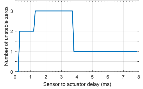
Fig. 2. Number of unstable zeros of PATO system for h = 8ms and D_c \in [0, h)
