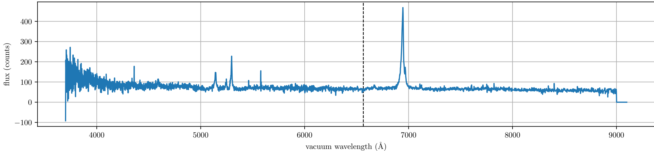
spec-56798-HD141746N331518M01_sp16-150.fits (LAMOST J141403.15+352311.3, Rmag: 17.11, label: double-peak, subclass: Non)
