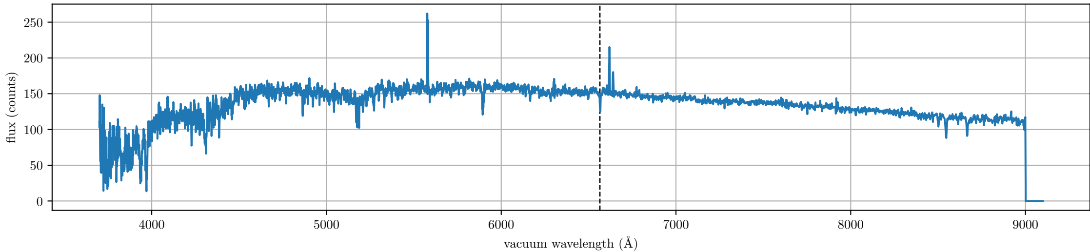
spec-56752-HD150254N020528B01_sp08-150.fits (LAMOST J150711.68+013202.4, Rmag: 16.37, label: double-peak, subclass: G8)
