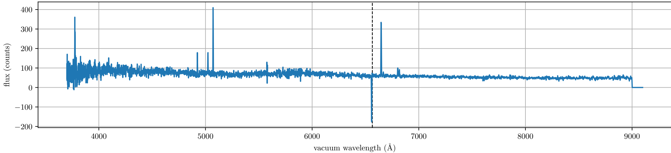
spec-56739-HD114047N212109B_sp10-131.fits (LAMOST J113114.00+211841.3, Rmag: 16.74, label: emission, subclass: Non)
