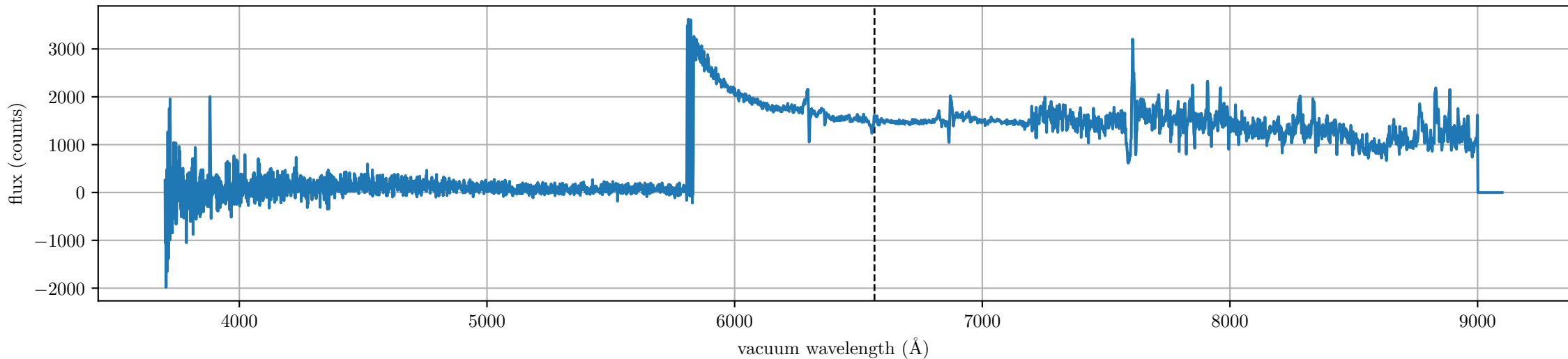
spec-56699-GAC085N52V3_sp15-178.fits (LAMOST J053944.81+531825.7, Rmag: 13.84, label: emission, subclass: Non)
