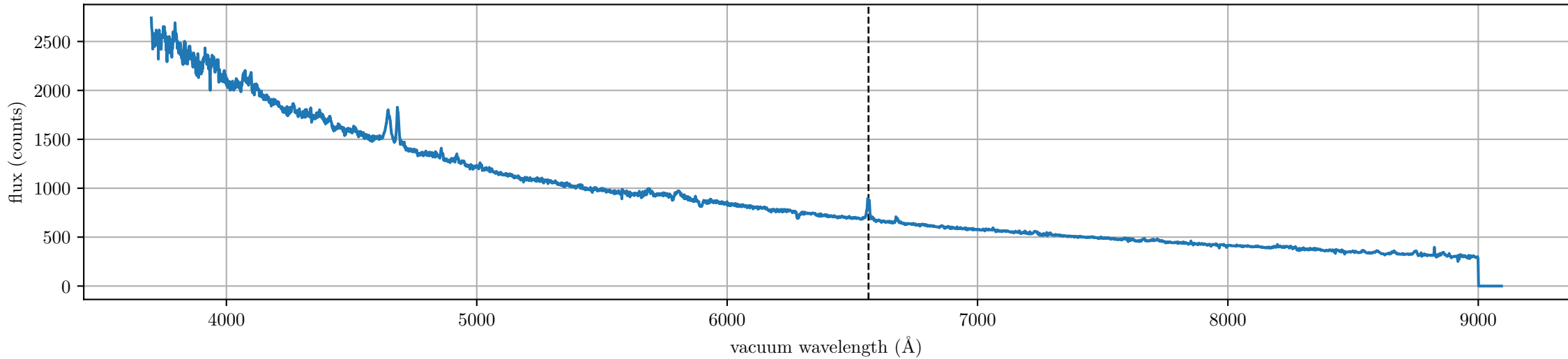
spec-56661-GAC061N34B1_sp07-028.fits (LAMOST J040901.83+323955.6, Rmag: 14.56, label: emission, subclass: K7)
