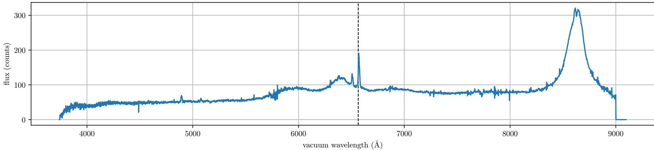
spec-56657-M31020N36M1_sp08-216.fits (LAMOST J012555.94+351036.9, Rmag: 16.08, label: emission, subclass: Non)
