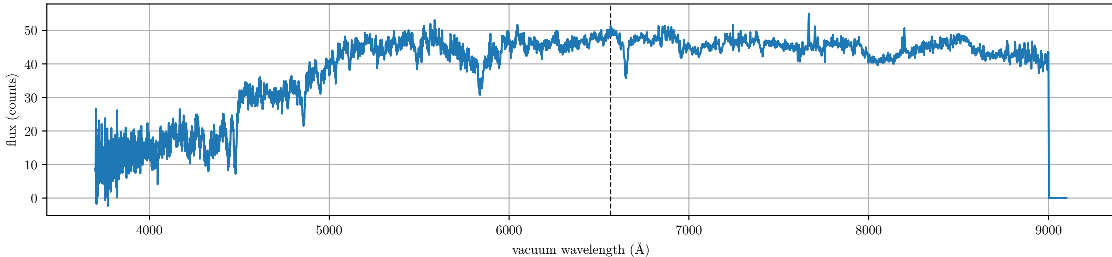
spec-56633-HD095000N333605M01_sp10-109.fits (LAMOST J093915.39+331634.2, Rmag: 16.36, label: emission, subclass: G2)
