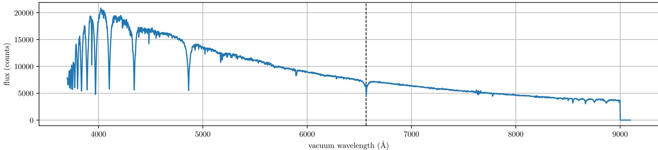
spec-56625-GAC113N37V1_sp07-098.fits (LAMOST J074244.51+353401.3, Rmag: 99.0, label: double-peak, subclass: A1IV)
