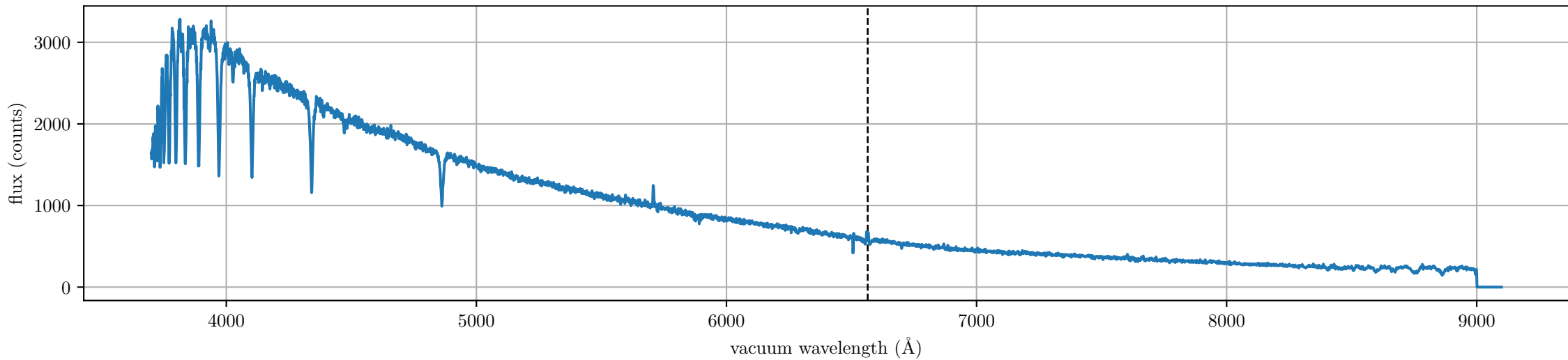
spec-56618-GAC105N47V2_sp10-151.fits (LAMOST J065632.72+461614.9, Rmag: 12.16, label: double-peak, subclass: B6)
