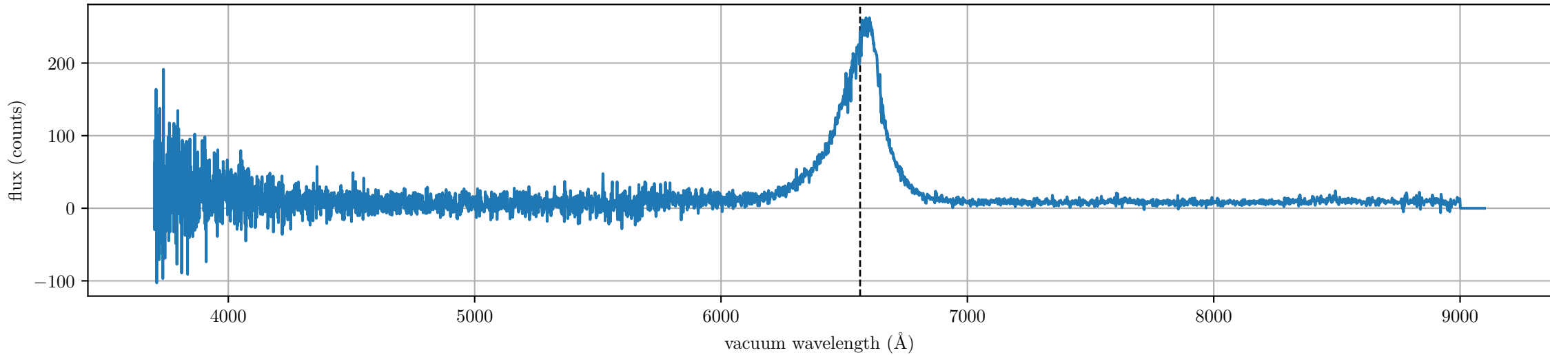
spec-56396-HD165712N321400M01_sp06-166.fits (LAMOST J170758.50+313441.1, Rmag: 14.36, label: emission, subclass: Non)
