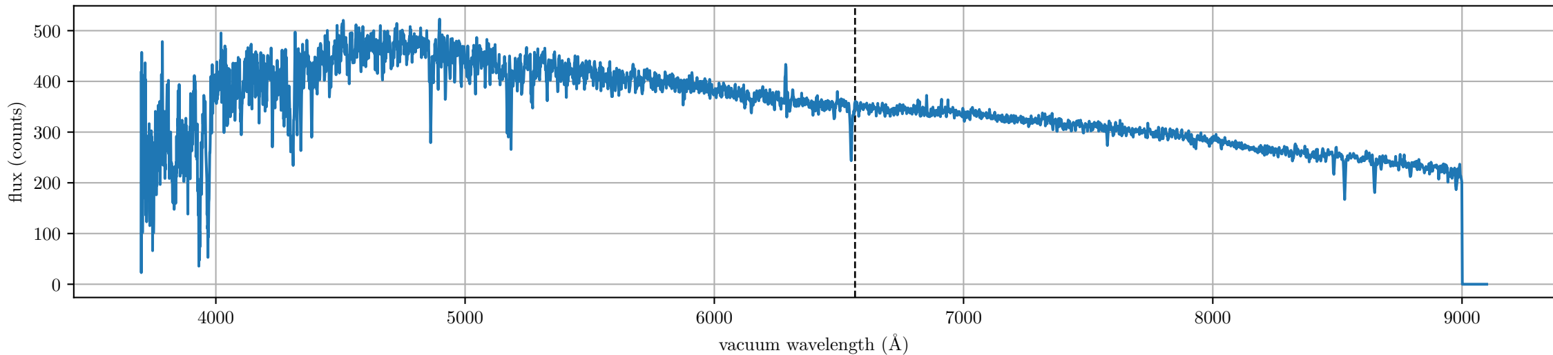
spec-56393-HD172143N395828M01_sp16-162.fits (LAMOST J171623.21+412303.1, Rmag: 14.79, label: emission, subclass: G7)
