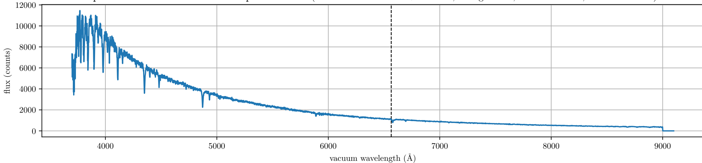
spec-56357-HD090901N073047B01_sp12-133.fits (LAMOST J091206.52+091621.8, Rmag: 13.22, label: emission, subclass: A0III)
