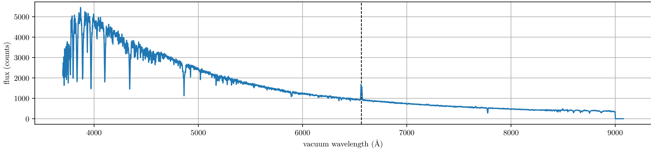
spec-56295-VB056N24V1_sp08-031.fits (LAMOST J034912.80+240820.0, Rmag: 13.36, label: double-peak, subclass: A3V)
