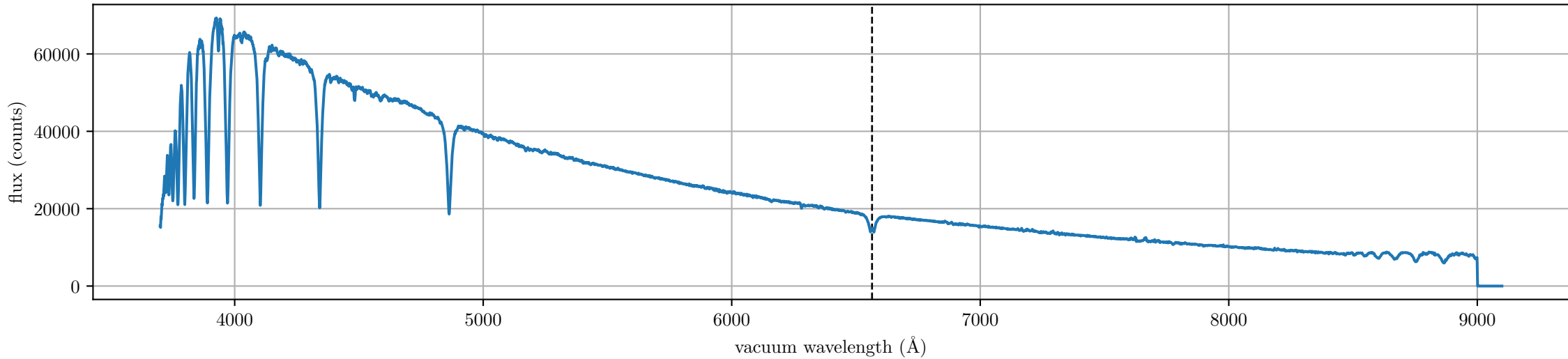
spec-56283-GAC120N18V2_sp15-115.fits (LAMOST J080032.50+185028.9, Rmag: 11.04, label: double-peak, subclass: A1V)
