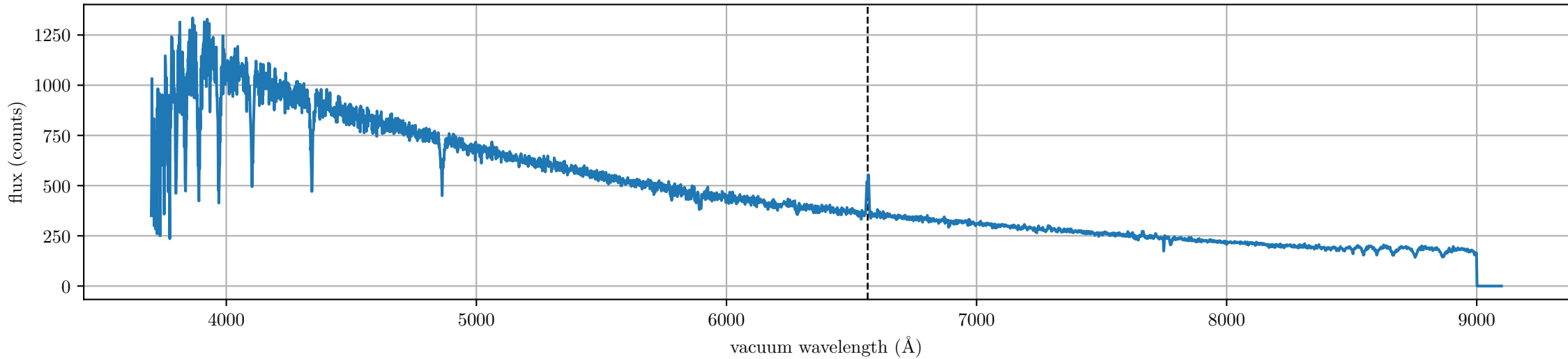
spec-56271-GAC084N26B1_sp10-057.fits (LAMOST J053040.90+260534.6, Rmag: 14.7, label: double-peak, subclass: A2V)
