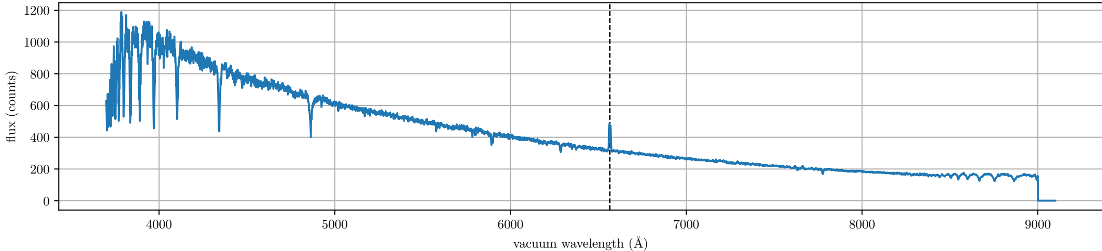
spec-56218-GAC083N27B2_sp02-234.fits (LAMOST J053040.90+260534.6, Rmag: 14.7, label: double-peak, subclass: B6)
