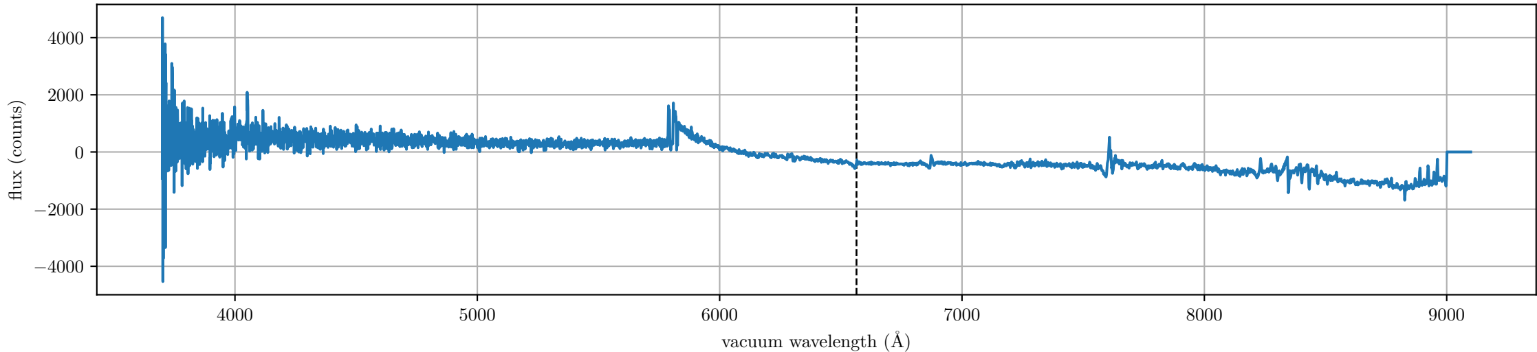
spec-56202-EG042015S023742V01_sp15-180.fits (LAMOST J041919.80-020211.6, Rmag: 14.65, label: double-peak, subclass: Non)
