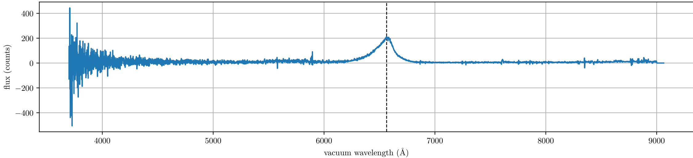
spec-56012-F5601204_sp02-158.fits (LAMOST J114009.42-012454.3, Rmag: 19.01, label: emission, subclass: Non)
