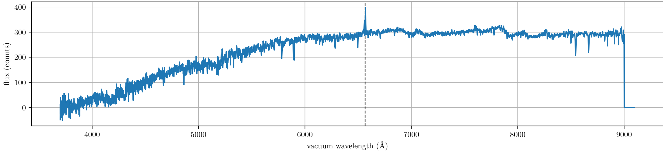
spec-55876-GAC_089N28_B2_sp04-121.fits (LAMOST J055821.00+284549.7, Rmag: 14.0, label: double-peak, subclass: K4)
