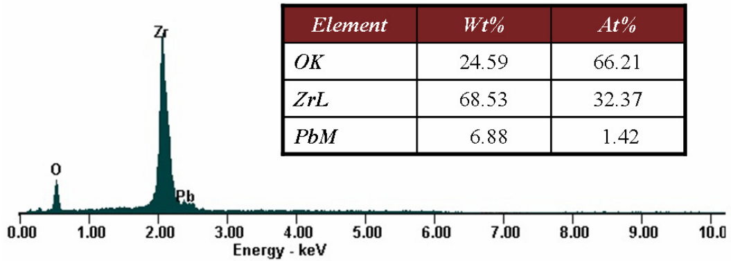
Figure 2. EDX data for MCN(single column fitting image)
