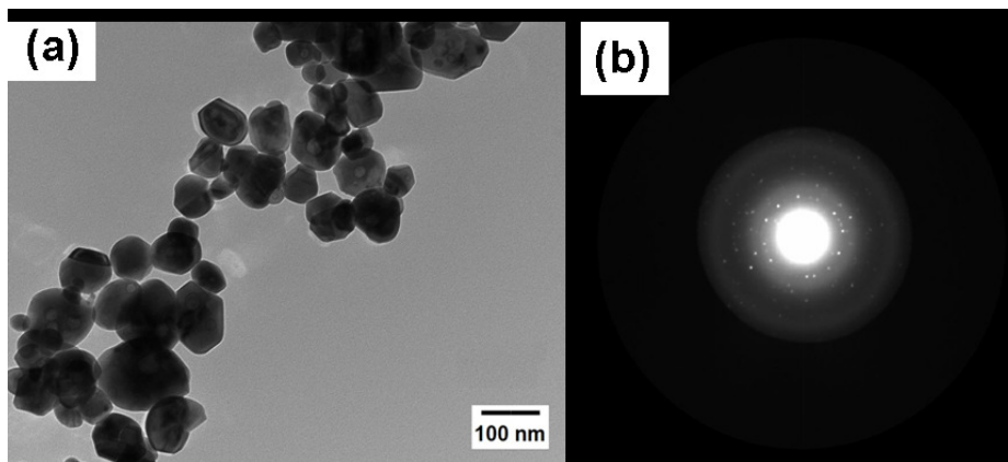
Figure 3. TEM analysis of the MCN: a) image of the nanoparticles; b) electron diffraction of the nanoparticles (2-column fitting image)
