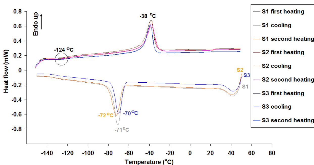
Figure 7. The differential scanning calorimetry curves for elastomers with MCN
