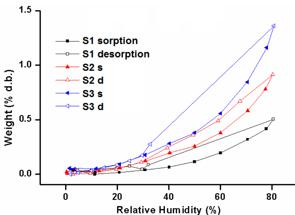
Figure 8. Dynamic vapour sorption isotherms for the elastomers containing ceramic nanoparticles (2-column fitting image)
