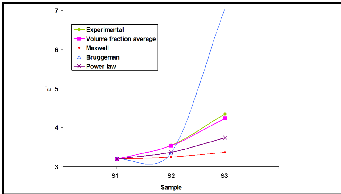
Figure 6. The values of the dielectric constant for the samples as determined experimentally in comparison with the values calculated with equations of different models
