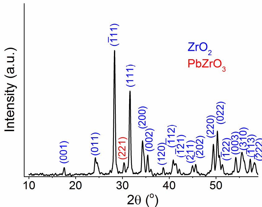
Figure 1. XRD patterns of the MCN powder (2-column fitting image)
