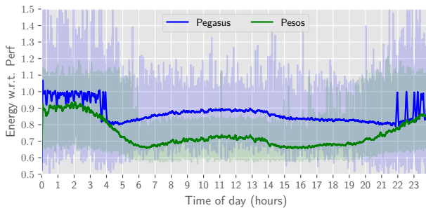
Figure 2: The CPU energy consumption of PEGASUS and PESOS w.r.t. PERF, both per second and with a order 3 Savitzky-Golay smoothing over a ten minutes time window.
