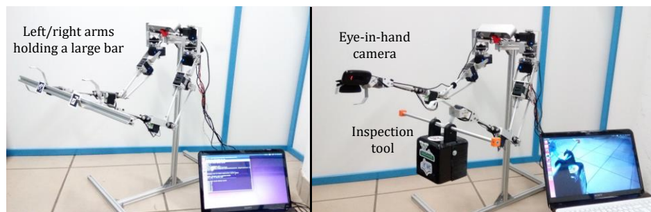
Fig. 2. Two illustrative application examples of the lightweight and human-size dual arm manipulator with ZED camera head.
