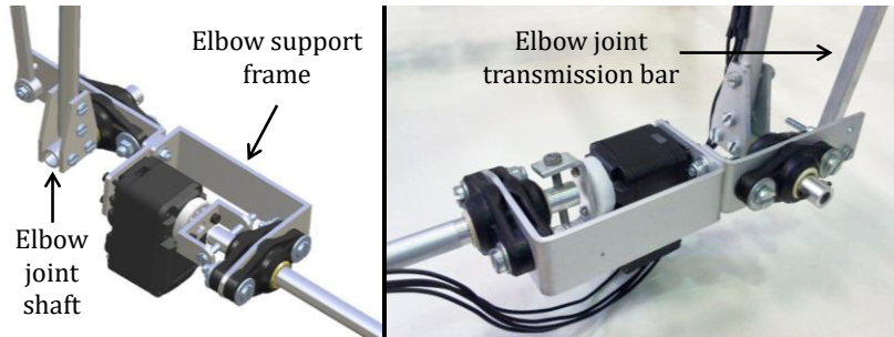
Fig. 4. Detailed view of the elbow joint mechanism and the wrist yaw servo. Radial loads exerted at the end effector are catch by the pair of igubal EFOM-08 bearings and supported by the aluminium frames.
