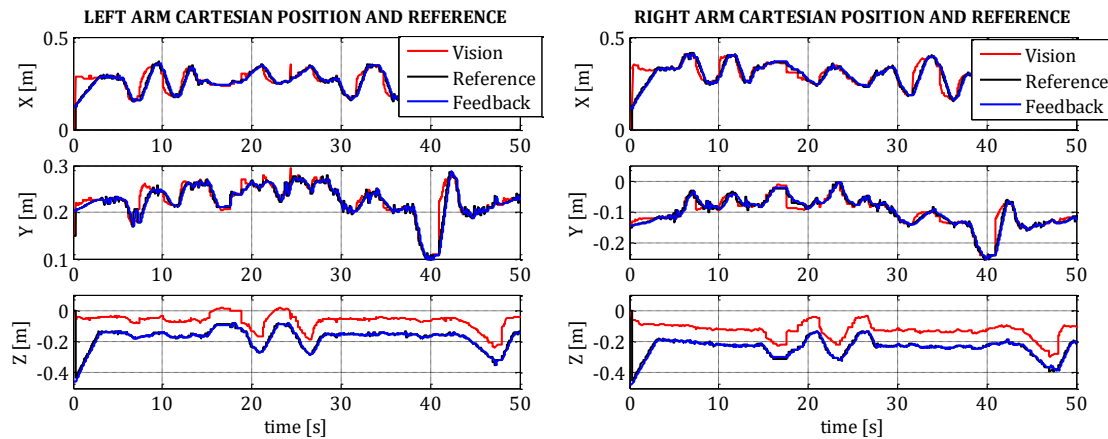
Fig. 19. Cartesian position of the left and right arms in the visual servoing experiment. Each arm tracked an ARUCO tag. An offset distance of 10 cm in the Z-axis was introduced for avoiding that the tags are occluded by the end effector.
