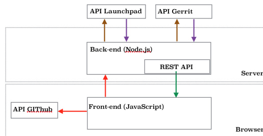
Fig. 1. Architecture of the tool.
