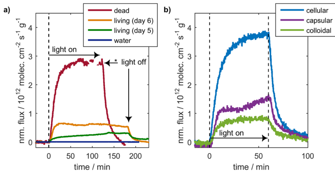
Fig. 2 Observed fluxes from PTR-MS measurements (normalized to biofilm dry-weight) upon sample irradiation for the sum of increasing signals (Table S-1) as a function of time: (a) Fluxes for autoclaved (i.e. dead) and authentic (i.e. living) biofilms for two different days. In addition, observed fluxes of a ground water experiment are given as background. (*Irradiation of the dead biofilm sample was stopped after 120 min, while the other samples were irradiated for 180 min.) (b) Normalized fluxes for the cellular, capsular, and colloidal fraction of a biofilm sample upon irradiation.
