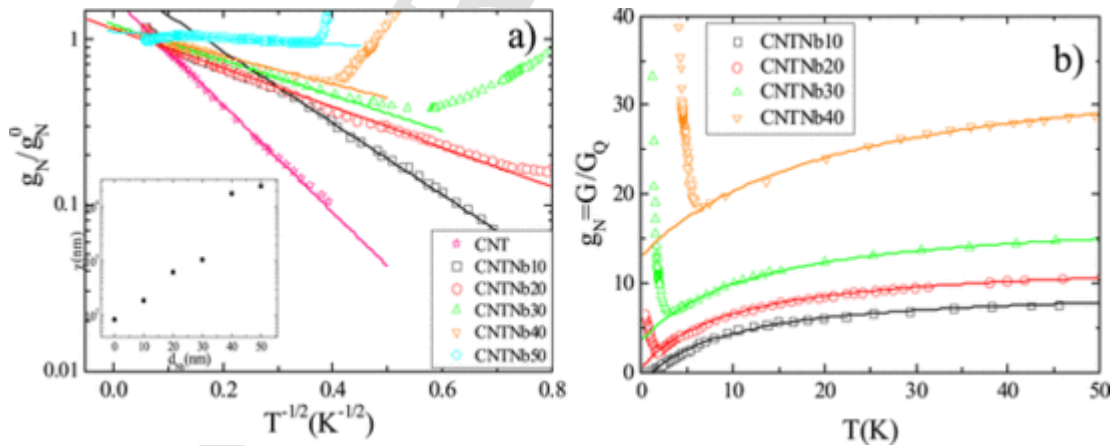
Fig. 4. a): Conductance normalized with respect to its value at T = 150 K, vs. 1/\sqrt{T} . The lines are fit to the data using Eq. (4). Inset: electron localization length \chi vs. d_{Nb} . -b): Temperature dependence of the normalized conductance. The lines are the best fit to the data obtained according to the diffusive Coulomb blockade model, Eq. (5). (A color version of this figure can be viewed online.)
