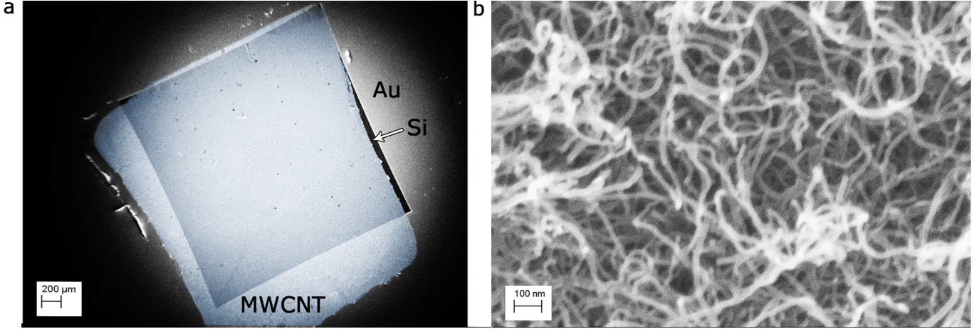
Figure 1: Scanning electron micrographs of a MWCNT film deposited on the solar cell Si substrate magnified at 65\times (a) and 200,000\times (b). a , The MWCNT film (light blue false color) deposited on Si active window (dark square area underneath the film) appears to be homogeneous and defect-free. b , At higher magnification the film exhibits a dense MWCNT random network.
