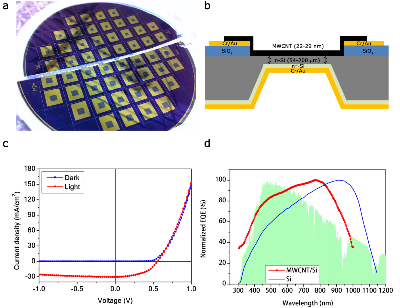
Figure 3: Device characterization. Photographic image of the device before the MWCNT film deposition (a) and sketch in cross section (b) of the MWCNT/Si solar cell. c, Electrical response of our best MWCNT/Si device under dark (blue dotted line) and under illumination (red dotted line). d, External quantum efficiency of our best device (red dotted line) as a comparison with that of a reference p-n Si solar cell (blue solid line) and the AM 1.5 G solar irradiance spectrum (green shaded area). Solar irradiance spectrum and EQEs are normalized to the maximum point.
