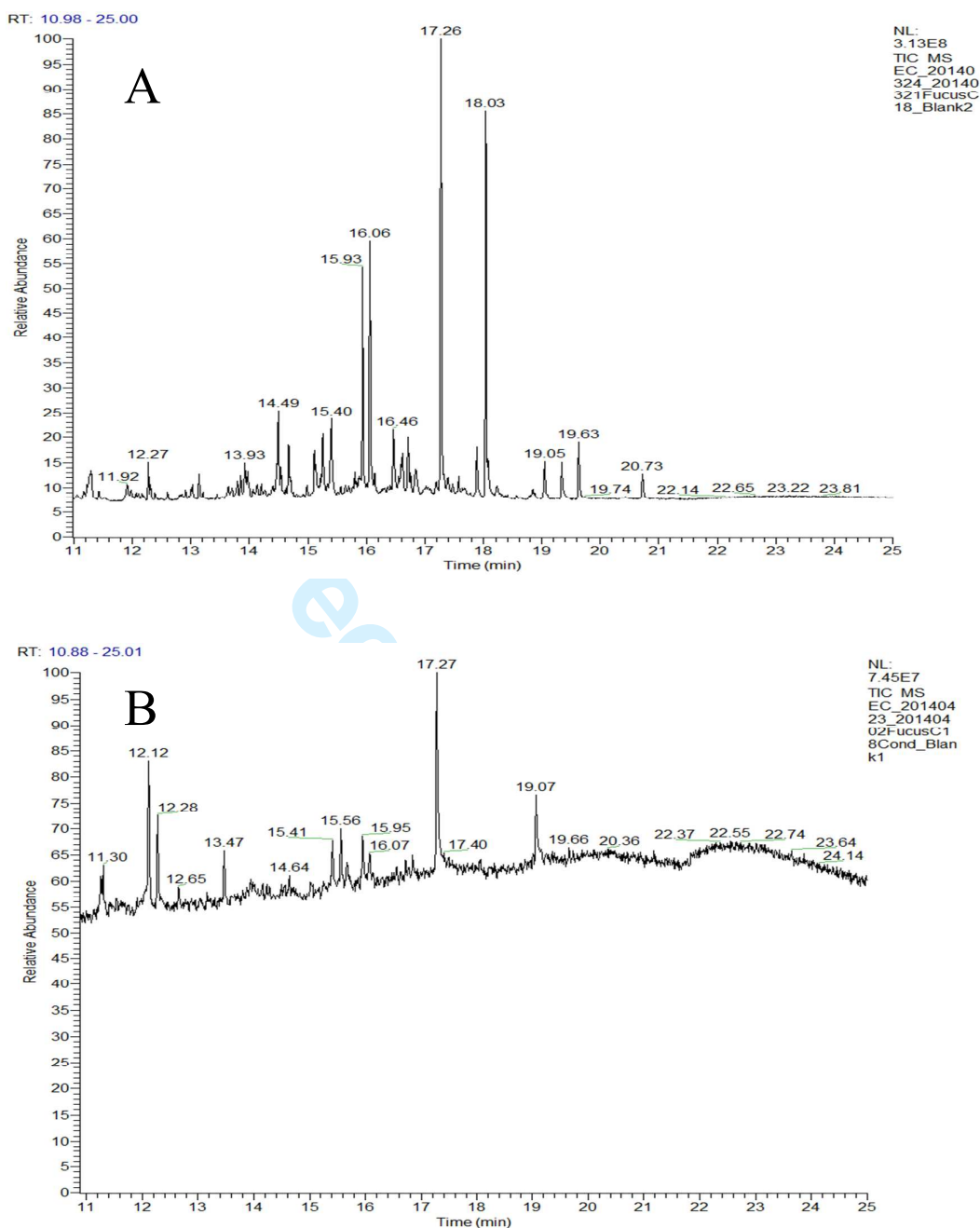
Figure S2: GC/MS profiles of C18 material (non endcapped) blank A) before and B) after conditioning with eluting solvent. All peaks did also show up in C18 surface extracts.
