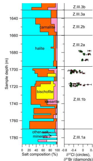
Figure 2: Left, stratigraphic column of drillhole TCI-2 indicating the average mineral composition of the salt minerals per interval. Other salt minerals indicate mainly sylvite and langbeinite. Right, measured \delta^{37}\text{Cl} (circles) and \delta^{81}\text{Br} (diamonds) values of the samples taken from the indicated depths. Both isotope systems are plotted in the same column so that it is easily visible that the isotope behaviour of Cl and Br depends on the mineralogical composition of the salt. Compared to samples analysed in the research by Eggenkamp et al. (1995) samples are not taken evenly over the length of the core but from sections dominated by halite, carnallite and bischofite in order to obtain characteristic isotope data for samples dominated by these minerals.
