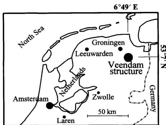
Figure 1: Location of the Veendam Salt Structure in the Netherlands (after Coeleweij et al., 1978).
