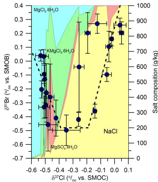
Figure 5: Relationships between \delta^{37}\text{Cl} , \delta^{81}\text{Br} and the mineralogical composition of the samples. Please note that the first precipitated salt is the salt with the highest \delta^{37}\text{Cl} value that is located on the right of the figure. Salt evolution evolved to the left in this figure.
