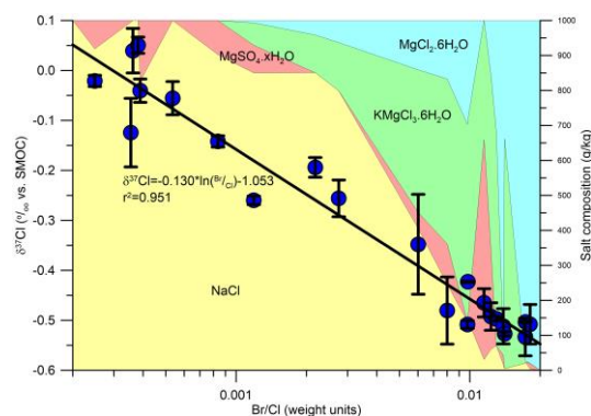
Figure 3: Relationships between \delta^{37}\text{Cl} , Br/Cl ratio and the mineralogical composition of the samples.
