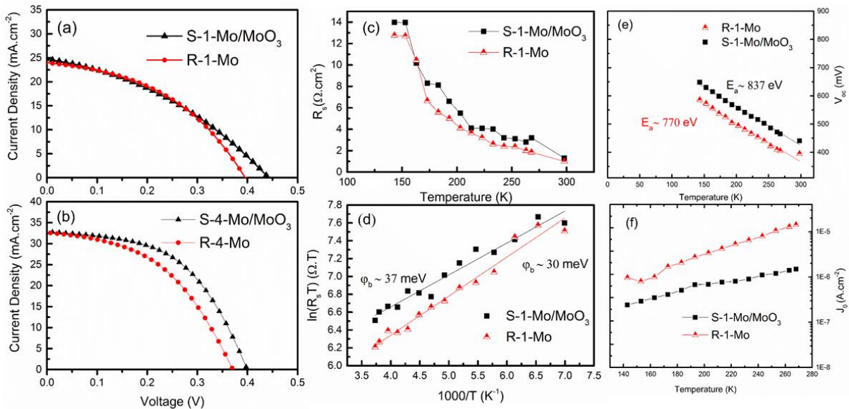
Figure 3 (a) AM 1.5 illuminated J-V curve of the champion solar cells with/without the MoO 3 layer of one of the thin samples (S/R-1) and (b) one of the thick samples (S/R-4). (c) Thermal behavior of series resistance ( R_s ), (d) Arrhenius plot of R_s , (e) Thermal behavior of V_{oc} and (f) ideality factor ( A )/dark saturation current ( J_0 ) of the best thin solar cells with/without MoO 3 layer (S-1/R-1).
