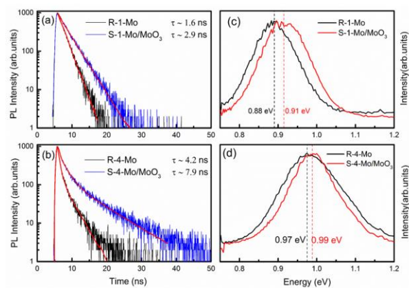
Figure 1 Room temperature TR-PL spectra of the samples with and without MoO 3 layer (a) thin samples and (b) thick samples. Room temperature PL spectra of (c) thin and (d) thick samples.
