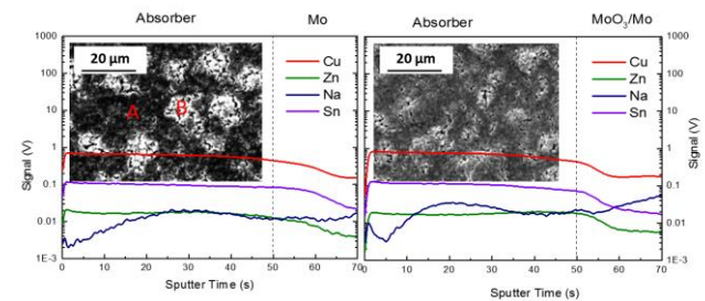
Figure 4 (left) GDOES measurements of sample R-4 (SLG/Mo/CZTSe) and (right) S-4 (SLG/Mo/MoO 3 /CZTSe). Sputter time = 0 s is the top surface of the CZTSe absorber layer.
