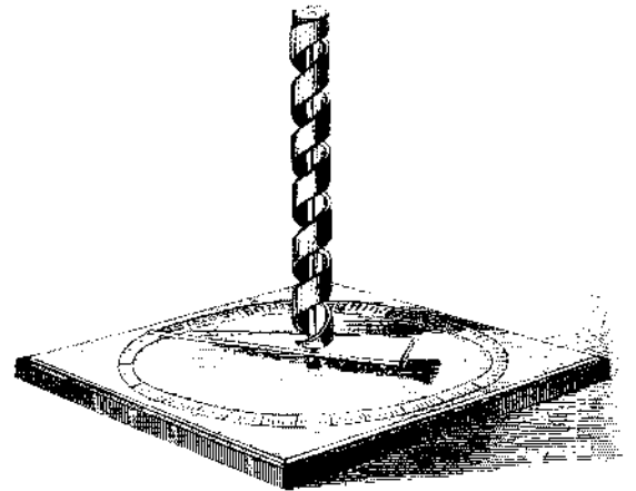
Fig. 1.—SIMPLE HYGROSCOPE.
