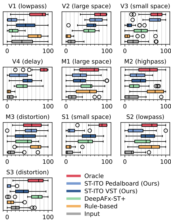
Figure 6. Subjective scores from N = 23 participants across vocals (V), music (M), and speech (S) examples.
