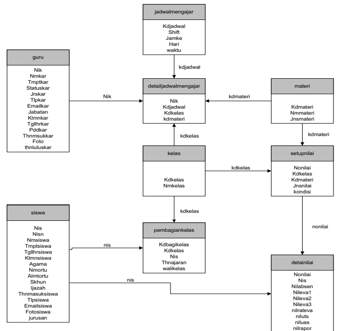
Gambar 9. Entity Relation Diagram
