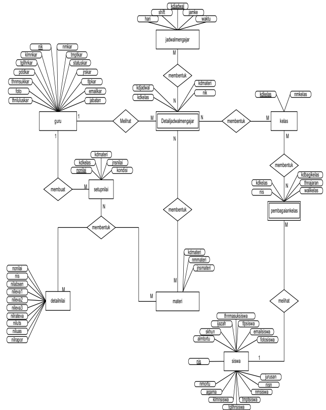
Gambar 8. Entity Relation Diagram
