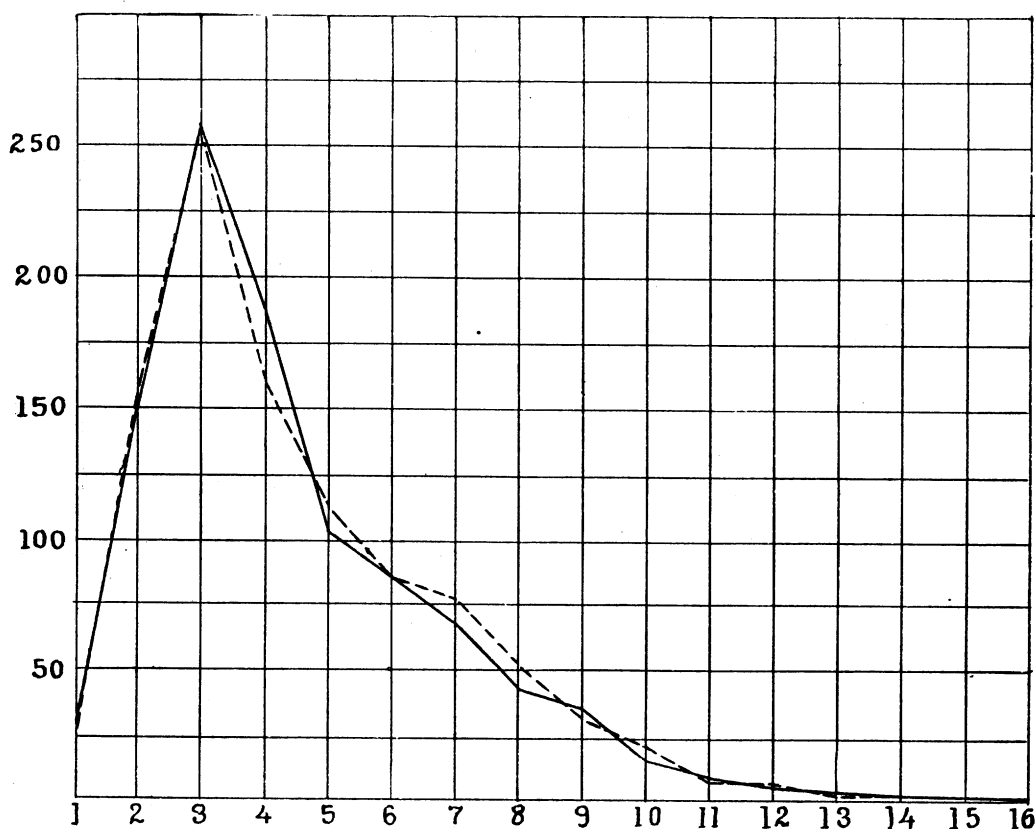
FIG. 6. — TWO GROUPS, OF FIVE THOUSAND WORDS EACH, FROM 'VANITY FAIR.'
