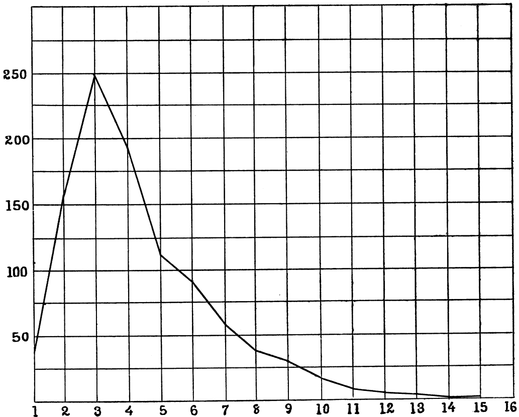
FIG. 5.—CURVE FOR TEN THOUSAND WORDS FROM 'OLIVER TWIST.'
