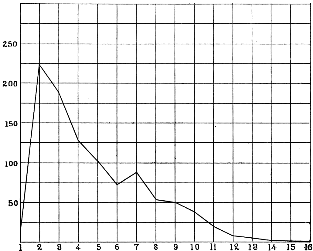
FIG. 9.—CURVE OF FIVE THOUSAND WORDS FROM MILL'S 'ESSAY ON LIBERTY.'
